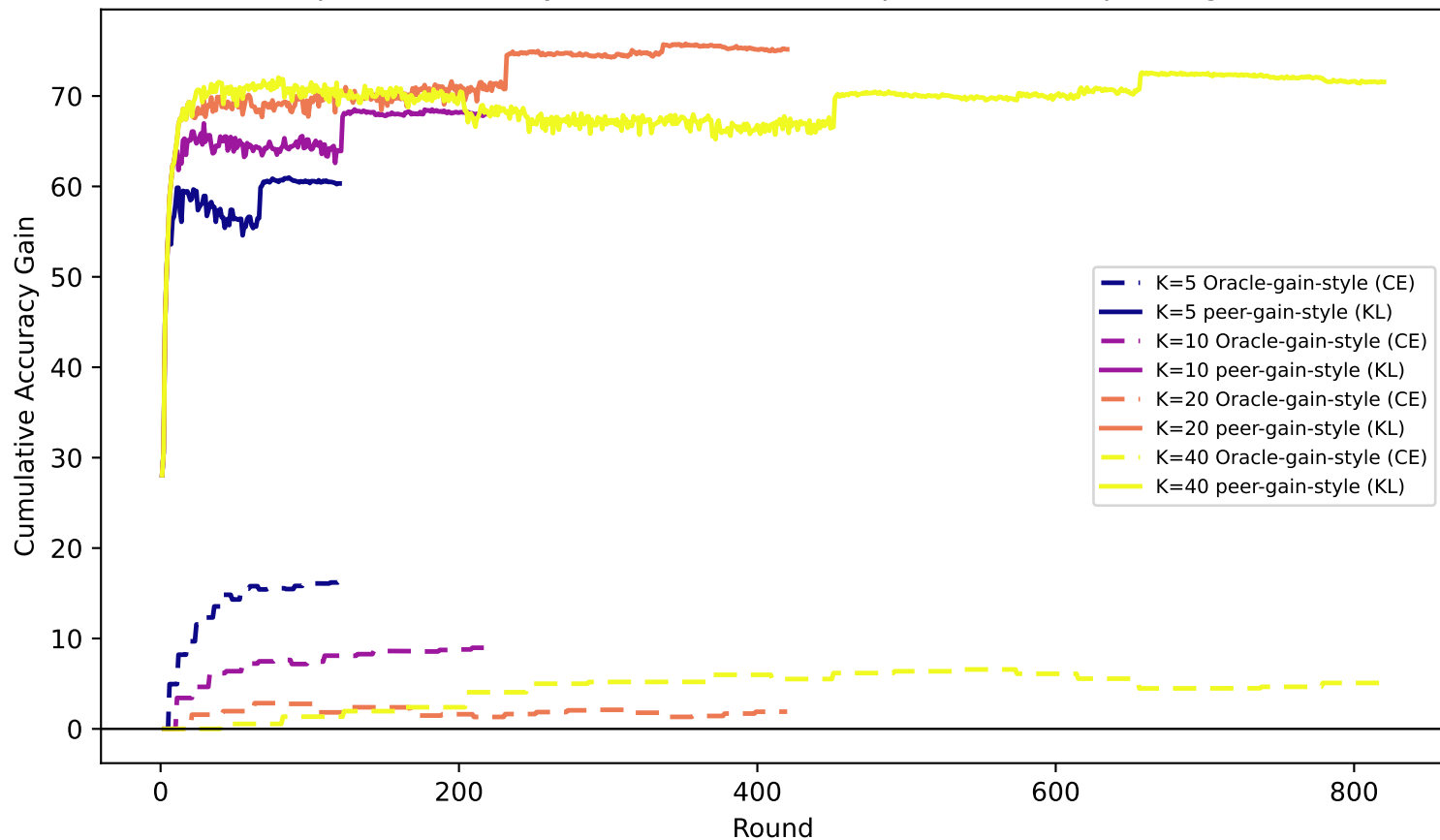
Repeated short-cycle: cumulative CE-update vs. KL-update gain
